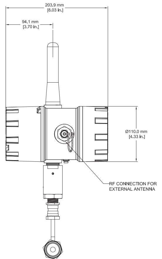
SIDE VIEW
