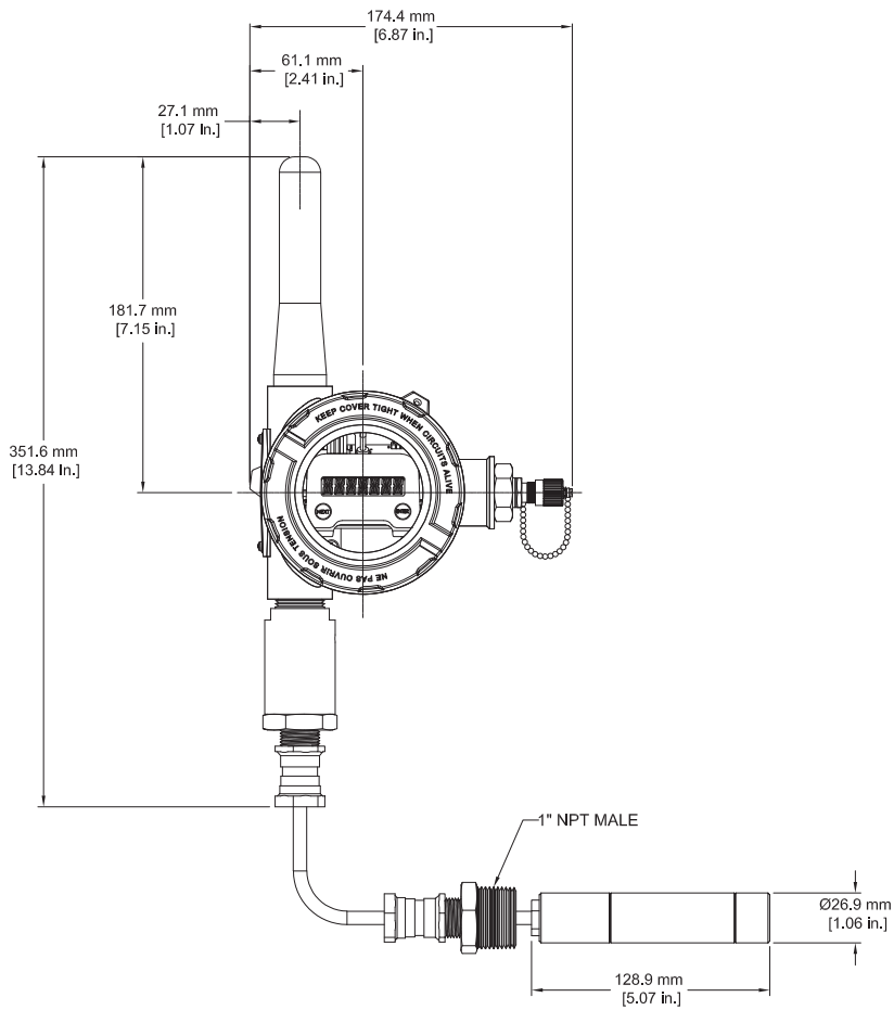
FRONT VIEW
