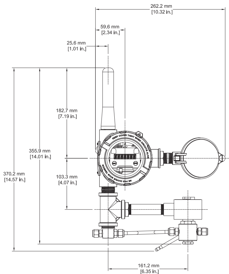
FRONT VIEW
